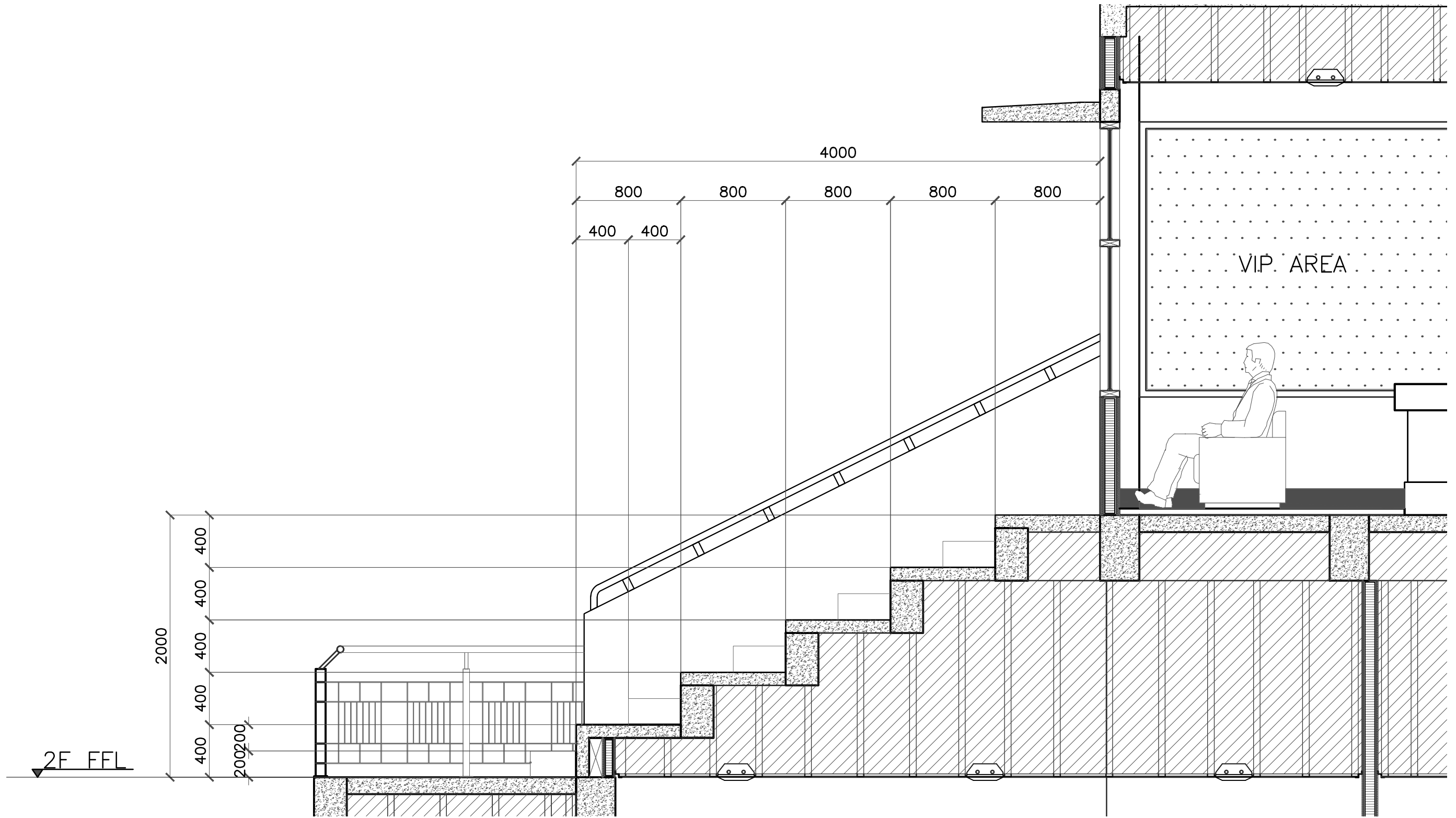
A BLEACHER SECTION 1 A-01 | A-01 SCALE 1:30 METERS
